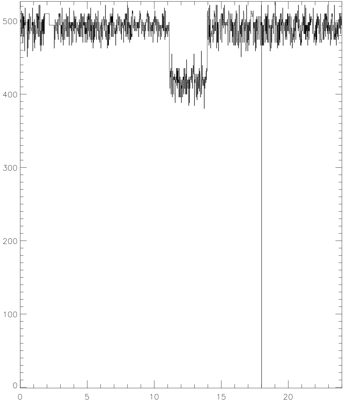
2000272 LVPS Current Monitor (mA)
