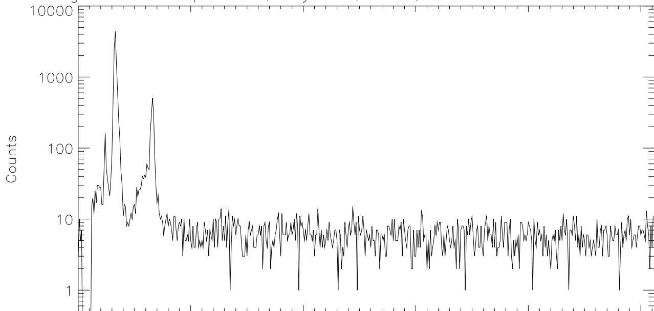
Figure 3a: ST spectrum, Day 128, 2001, 08:00–09:00 840–1120 eV
