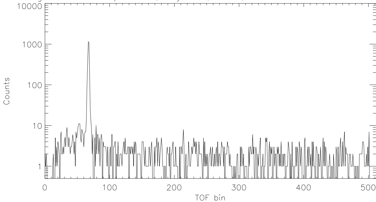
Figure 3b: LEF spectrum, Day 128, 2001, 08:00–09:00 840–1120 eV
